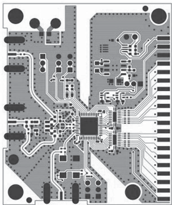
Silkscreen Topside
